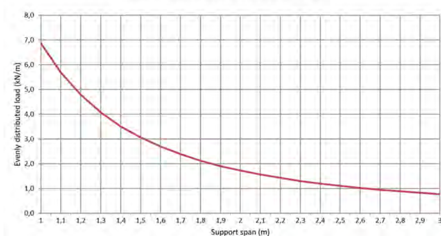
Permissible load KLA 100/600 d=2,0mm (kN/m)
