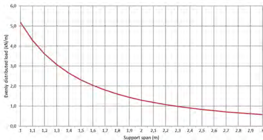
Permissible load KLA 60/600 d=2,0mm (kN/m)
