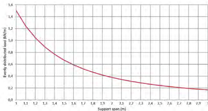
Permissible load KPA 60/200 d=1,0mm (kN/m)
