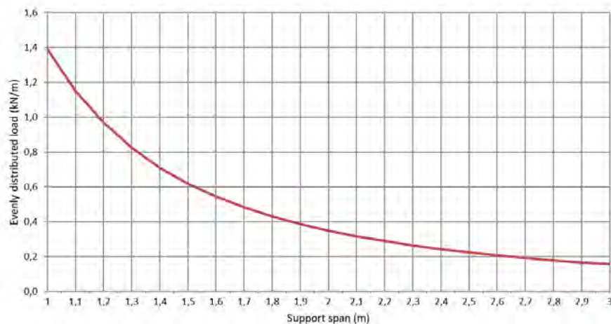
Permissible load KPA 60/300 d=1,0mm (kN/m)
