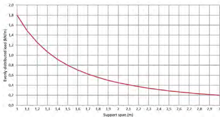
Permissible load KPA 60/400 d=1,0mm (kN/m)
