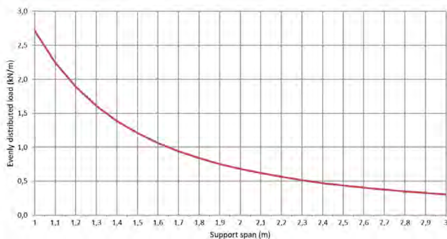
Permissible load KP 60/100 d=0,75mm (kN/m)
