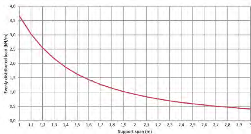
Permissible load KP 60/200 d=0,75mm (kN/m)
