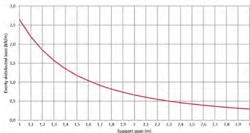
Permissible load KP 60/300 d=0,75mm (kN/m)
