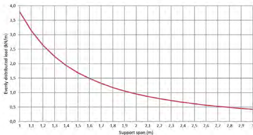
Permissible load KP 60/400 d=0,9mm (kN/m)
