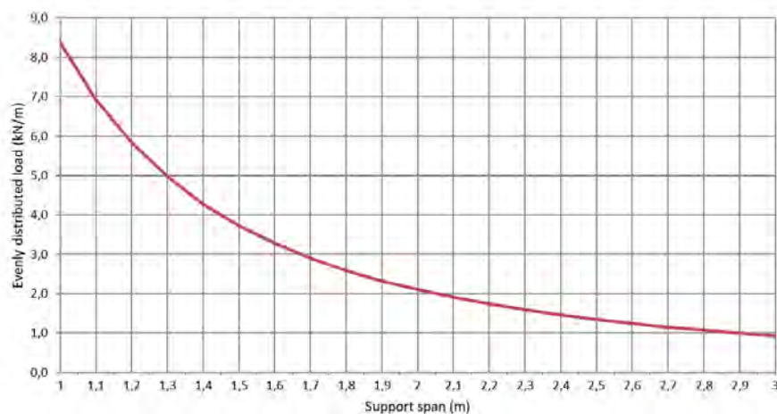
Permissible load KP 60/200 d=1,5mm (kN/m)
