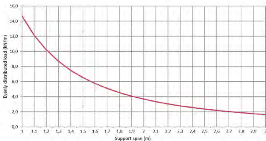
Permissible load KP 60/500 d=1,5mm (kN/m)
