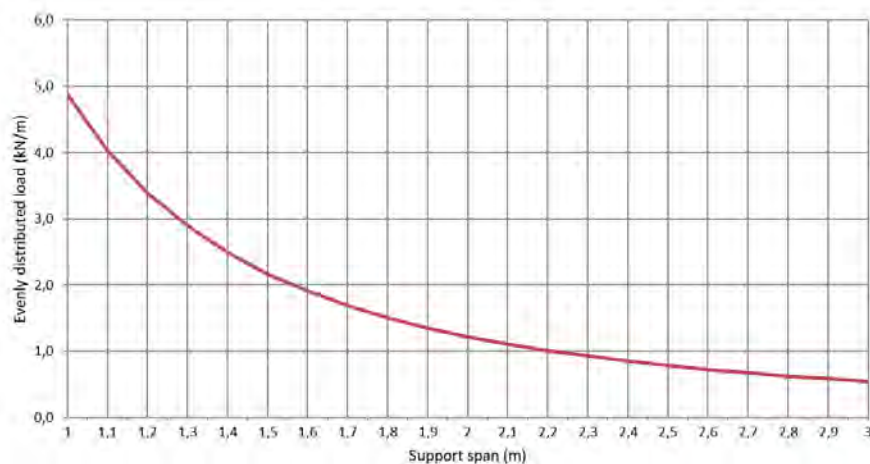
Permissible load KP 100/300 d=1,0mm (kN/m)
