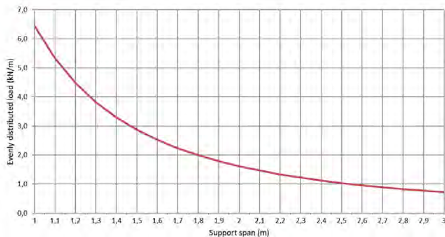
Permissible load KP 100/400 d=1,0mm (kN/m)
