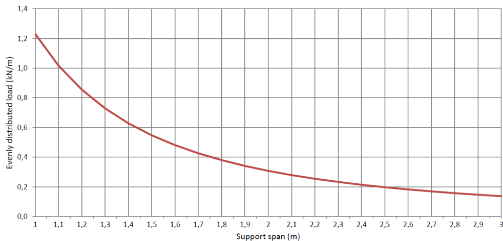
Permissible load KPK 60/100 d=0,6mm (kN/m)
