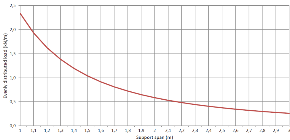
Permissible load KPK 60/100 d=0,75mm (kN/m)
